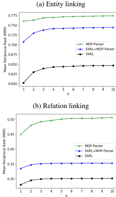
Figure 4. Performance in terms of MRR w.r.t. the value of k .
