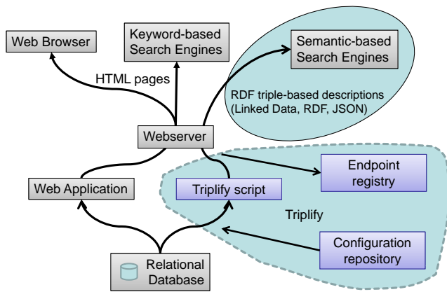
Figure 2: Triplify overview: the Triplify script is accompanied with a configuration repository and an endpoint registry.
