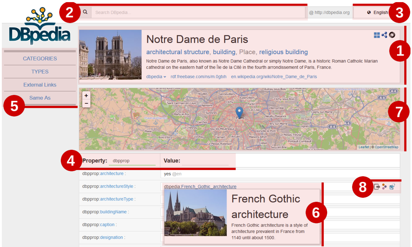
Figure 1: Screenshot of the new interface. The transparent red areas highlight new features, with the associated number in the red circle corresponding to its subsection number within Section 3. A quick overview: (1) pretty box, (2) search bar, (3) language switcher, (4) triple filter, (5) shortcuts, (6) preview box, (7) map and (8) triple actions.
