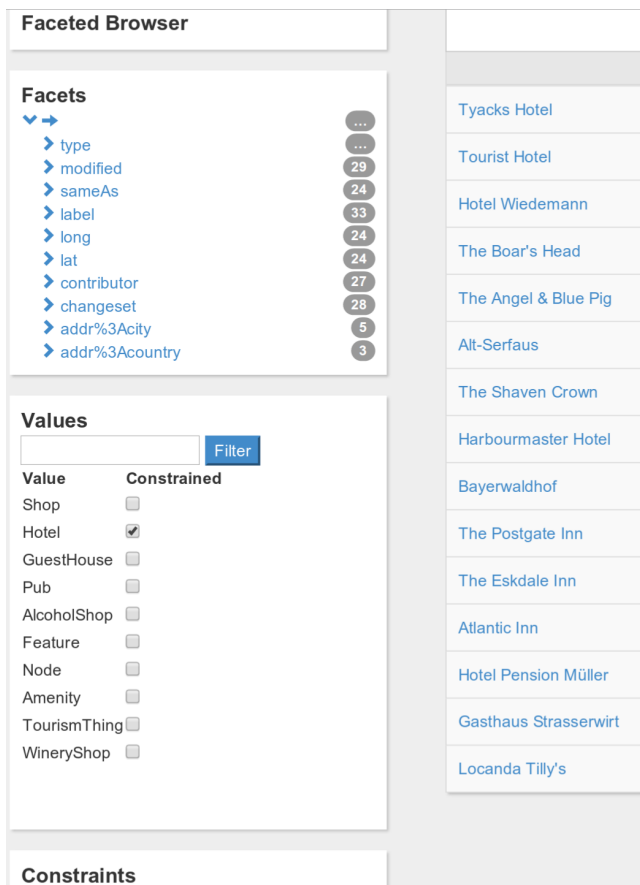
Figure 2: Screenshot showing the faceted browsing facilities for the class Pub at LinkedGeoData. A constraint has been set which restricts the pubs to those that are additionally typed as Hotel .
